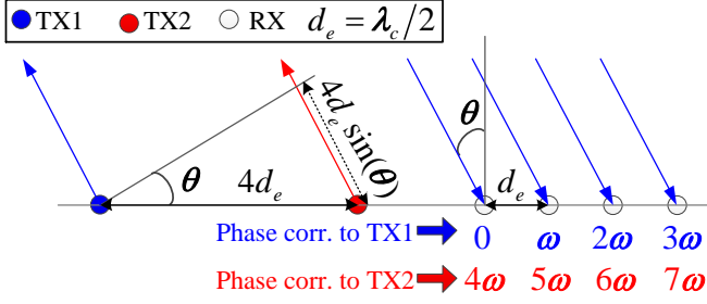
Fig. 3: Antenna Deployment.
