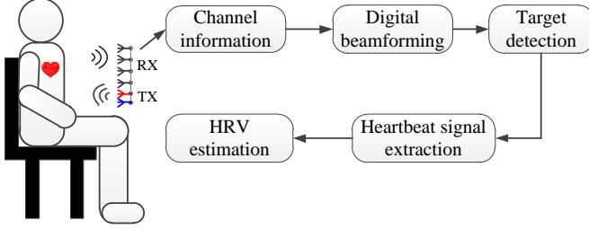
Fig. 1: Processing flow of mmHRV.
