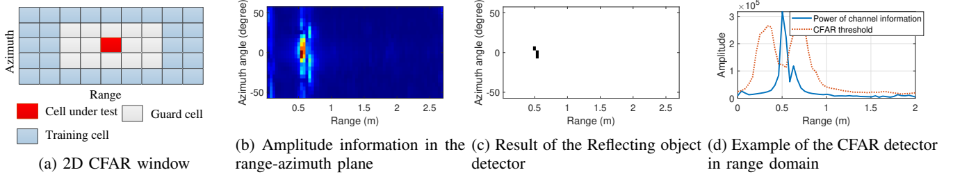
Fig. 4: Example of the reflecting object detector. The ground truth is that there is a human subject sit at 0.5m away from the device, with azimuth angle 0^\circ . (a) is the 2D-CFAR window, (b) is the amplitude of channel information in the range-azimuth plane, (c) is the reflecting result of reflecting object detector, where the black spot corresponding to the reflecting object, and (d) shows the CFAR threshold and the amplitude of channel information in range domain.
