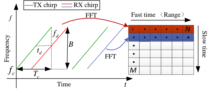
Fig. 2: FMCW radar system.
