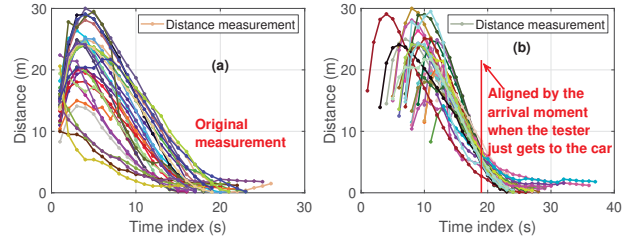
Fig. 6: Distance measurements in which the ISTA moves to the RSTA slowly (the tester walks slowly to the car).
