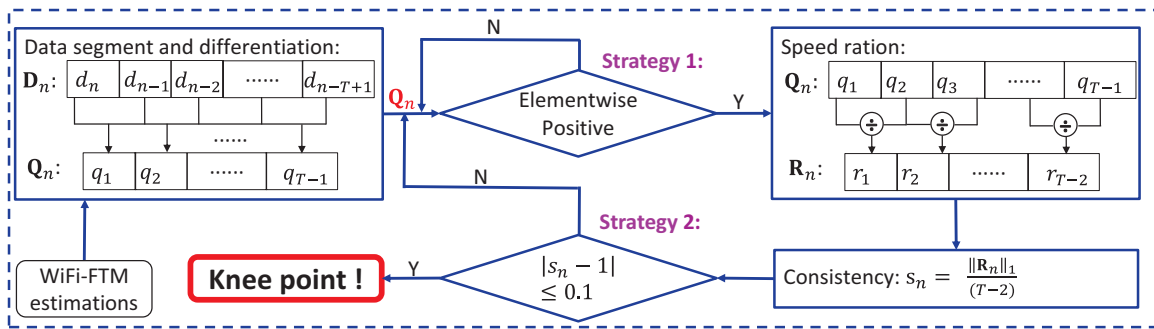
Fig. 7: Key steps of the knee point detection
